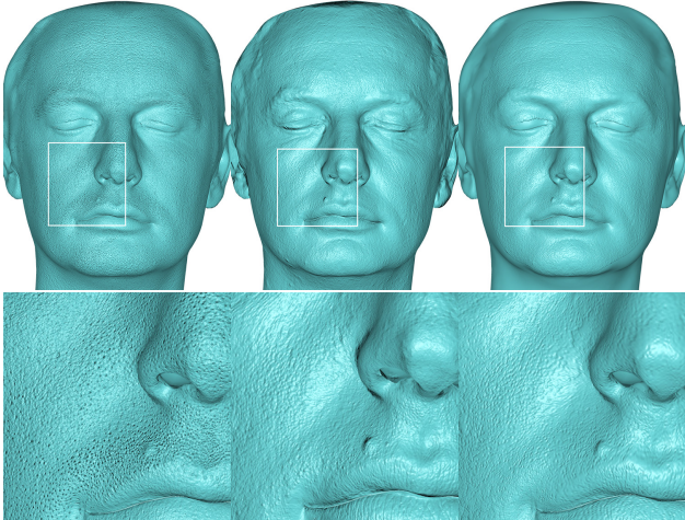
(a) Beeler et al.[6] (b) Ground truth [20] (c) our method
